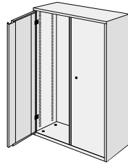
M181D H1880 x W1000 x D475
