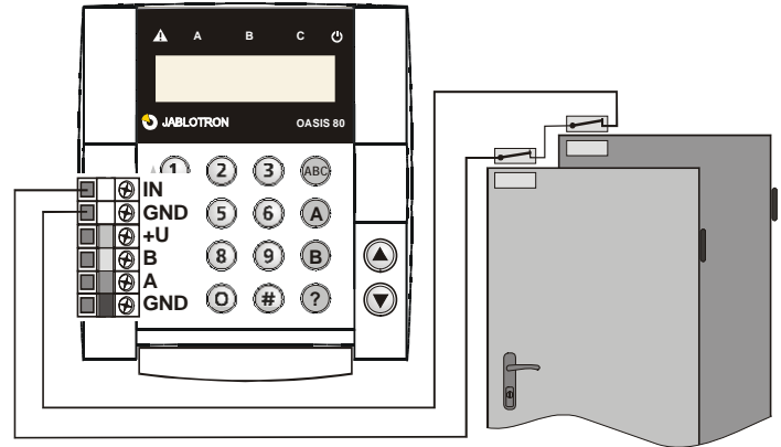
An example of door detector wiring
